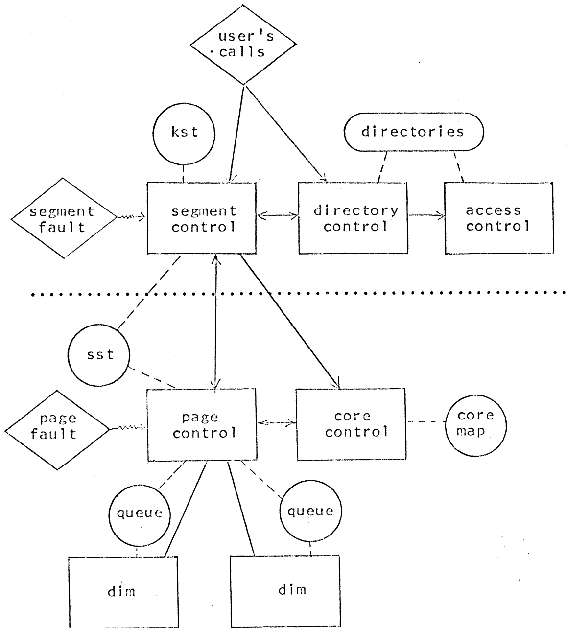
Figure 1. The Basic File System
